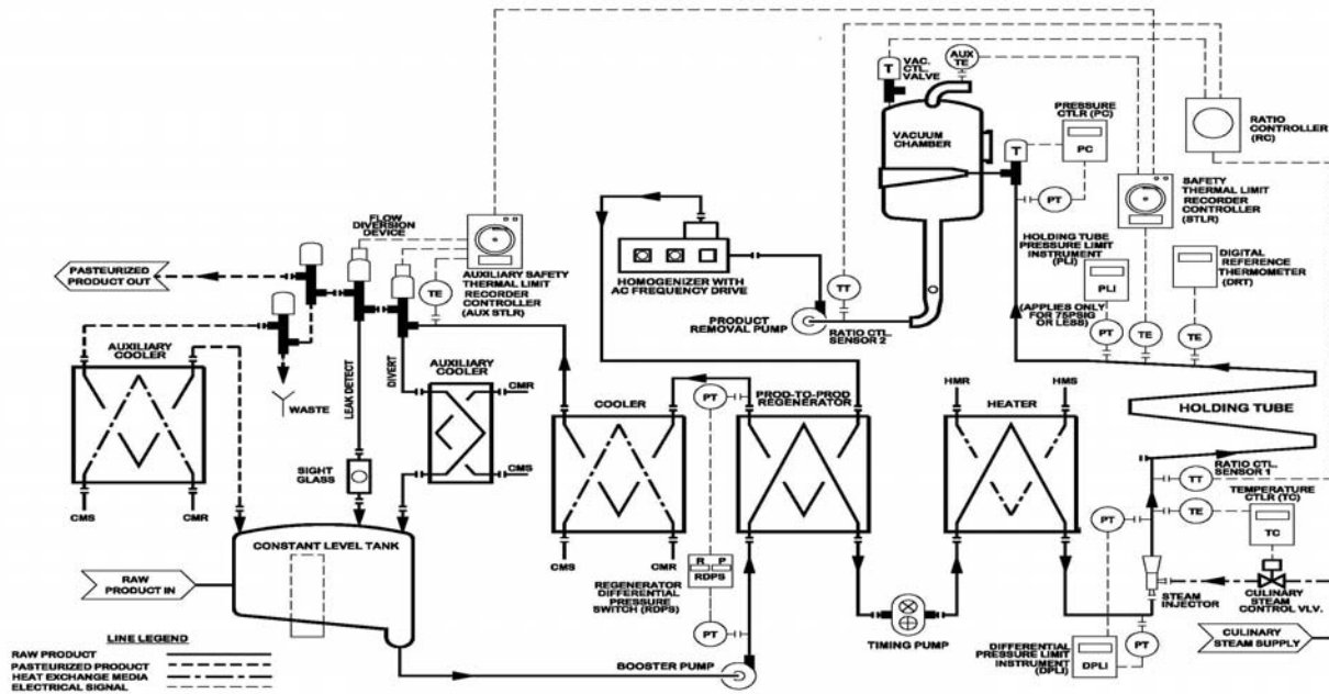
Figure 41. HHST Pasteurizer Utilizing Steam Injection Heating, Vacuum Flash Cooling and a Flow-Diversion Device Located Downstream of the Cooler Section
