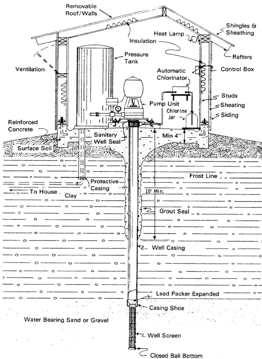
Figure 16. Pumphouse
