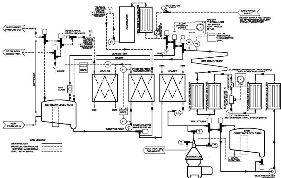
Figure 39. HTST Pasteurizer with a Regenerator, Separator, Skim Surge Tank and a Meter Based Timing System Located Upstream from an Evaporator
