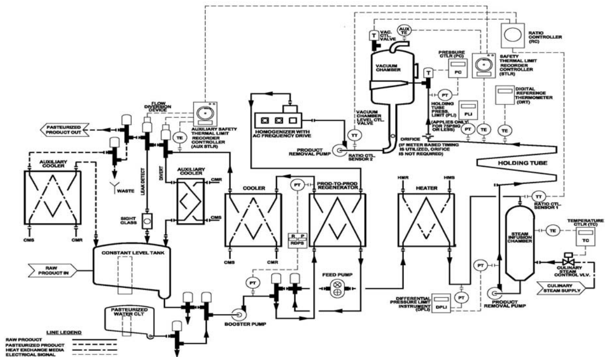
Figure 42. HHST Pasteurizer Utilizing Direct Culinary Steam Infusion and Vacuum Flash Cooling with a Homogenizer Located Downstream
